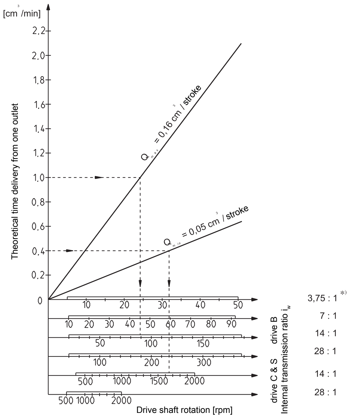
Fig. 3 Diagram of time delivery of pumps MPS 10-2 type, with drive B, C, S
