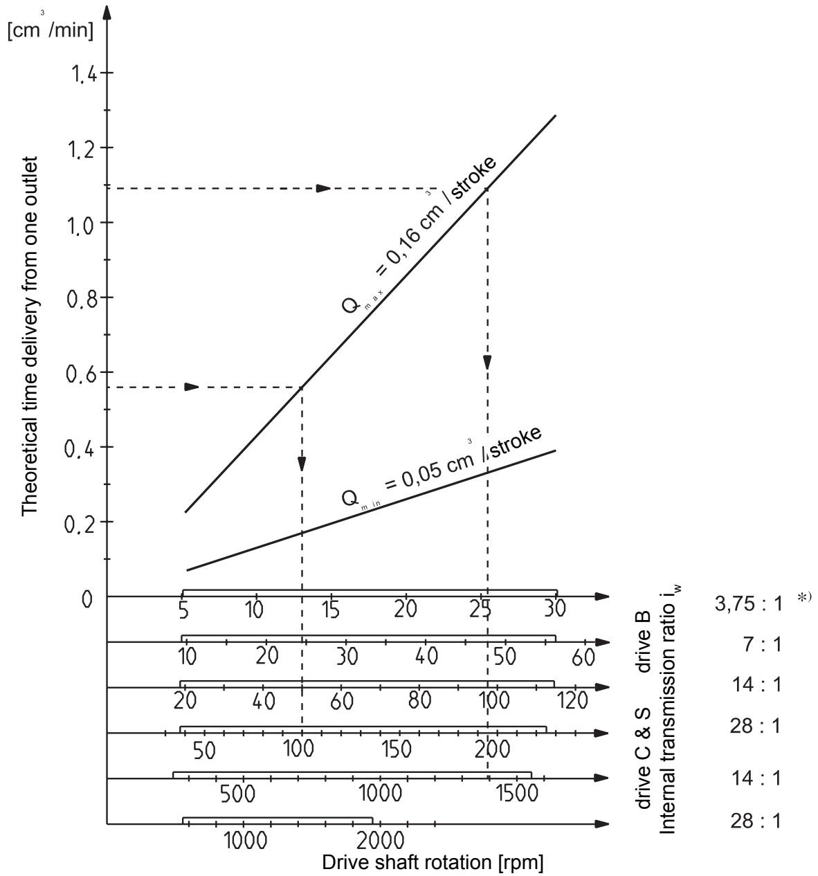
Fig. 2 Diagram of time delivery of pumps MPS 10-1 type, with drive B, C, S
